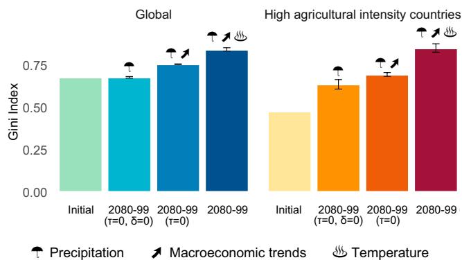
Fig. 4. Evolution of income inequality (Gini coefficients), globally and for high-agricultural-intensity countries, under different scenarios. The “2080-99 ( \tau = 0 , \delta = 0 )” scenario accounts for precipitation changes alone. The “2080-99 ( \tau = 0 )” scenario accounts for precipitation changes along with trends in per capita GDP and agricultural employment shares. The “2080-99 ( \tau = 0 , \delta = 0 )” scenario additionally accounts for temperature changes. Initial refers to historical averages (1991 through 2010). Multiplying projected bottom-50%-income shares by projected per capita GDP, we retrieve the per capita income for classes below and above the median (bottom 50% and top 50%), under the assumption of GDP being distributed as pretax national income. Gini coefficients are computed for each climate model and then averaged; they account for both within- and between-country income distribution. Error bars show 95% confidence bands. Two outlier countries (Bosnia and Herzegovina [BA] and Equatorial Guinea [EQ]) with highest average historical per capita GDP growth rates are excluded from the calculation.
